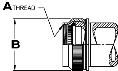
Style A, R & S INTERFACE PER MIL-DTL-81511 FIGURE 12C
