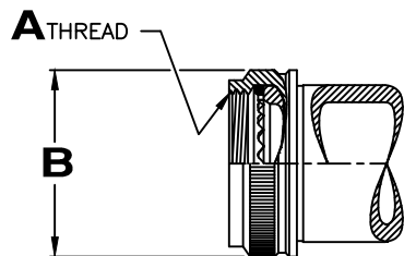
Style A, R & S INTERFACE PER SAE AS85049 FIGURE 2
