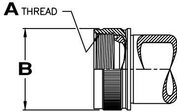
Style A, R & S INTERFACE PER SAE AS85049 FIGURE 4 O'RING NOT REQUIRED / SUPPLIED
