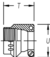
STYLE 4 △ STRAIN RELIEF ENVIRONMENTAL (AS85049/2) (MS 3057.**C)
